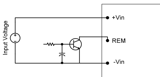
Figure9. Remote On/Off Implementation
