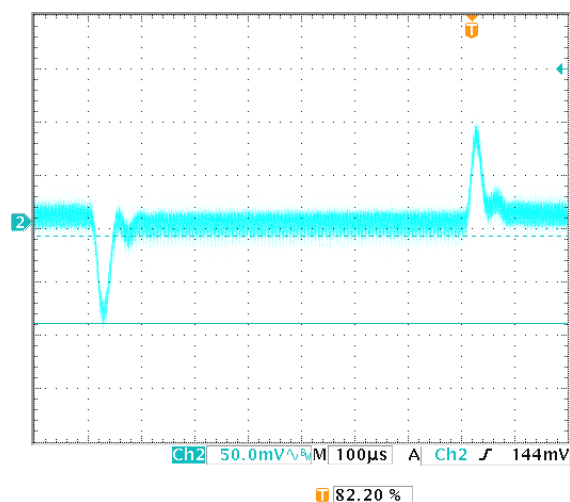
Figure4. Vin=48V, 50%-75%-50% load, 2.5A/μs@25°C
