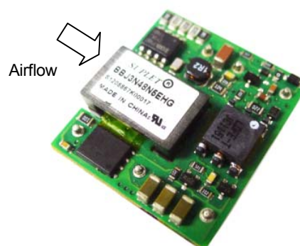
Figure13. Recommended Airflow Direction
