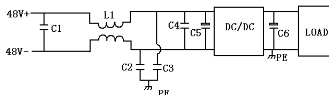
Figure15. Recommended EMC application
