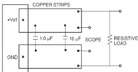
Figure8. Output Ripple and Noise Test Setup
