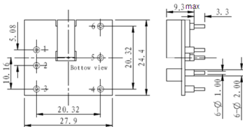
Figure16. Outline Diagram
