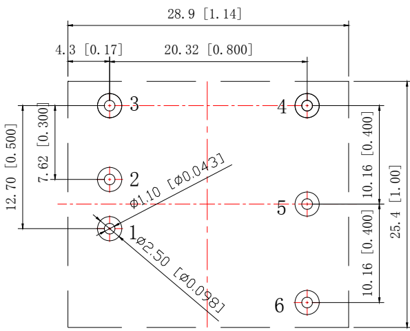
Figure17. Recommended Pad Layout
