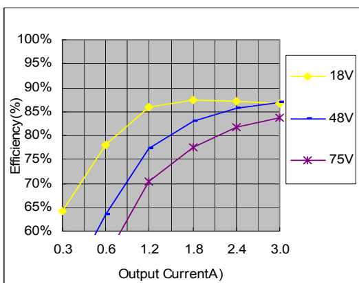
Figure1. Converter Efficiency Vs. Output Current@25°C
