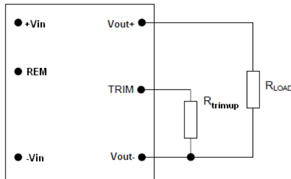
Figure10. Circuit Configuration to Increase Output Voltage
