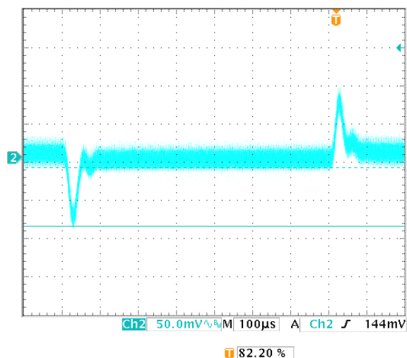
Figure3. Vin=48V, 25%-50%-25% load, 2.5A/μs@25°C
