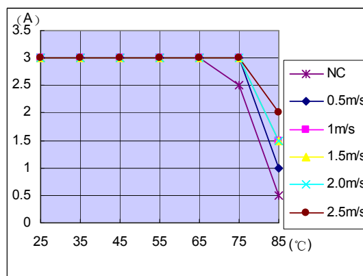
Figure2. Available load current Vs. ambient temperature and airflow for the module mounted horizontally
